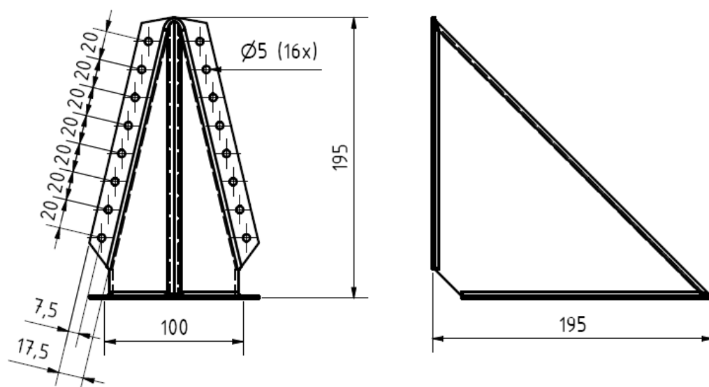
Figure B.4 Dimensions of Cleat 4213
